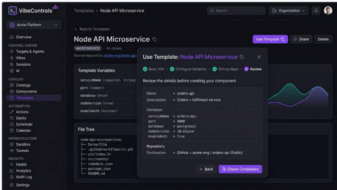
031 Template Scaffold Wizard
