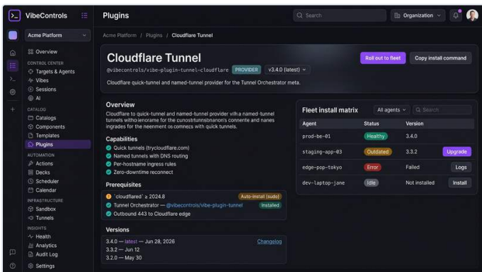
033 Plugin Detail Matrix
